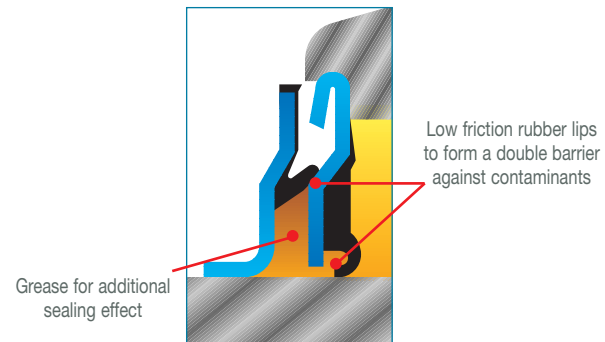
2RF SEALING SYSTEMS: SUPERAGRISEAL + RUBBERIZED FLINGER
