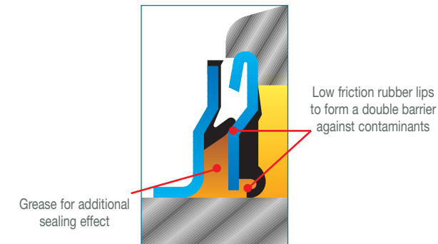
2RF SEALING SYSTEMS: SUPERAGRISEAL + RUBBERIZED FLINGER
